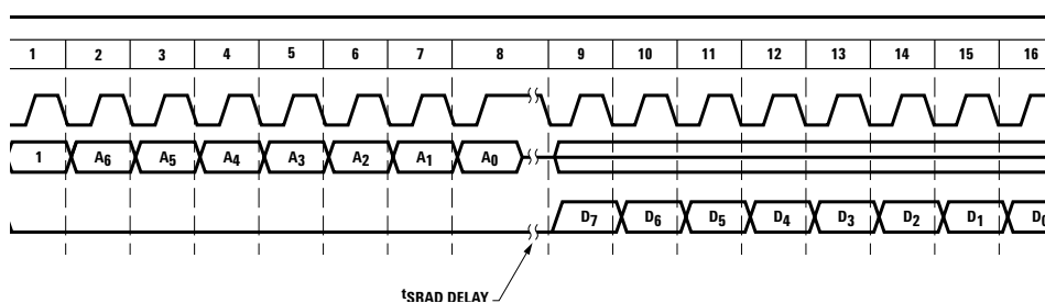
Figure 13. Read operation
