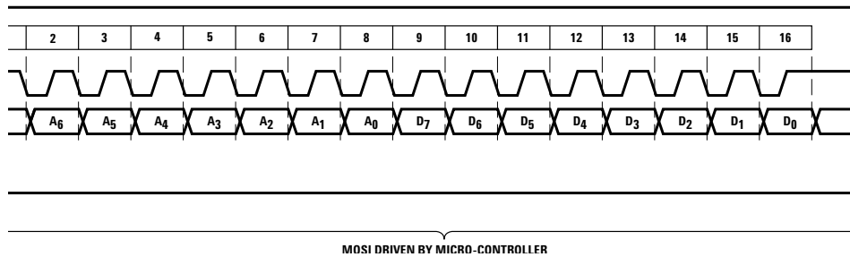
Figure 11. Write operation
